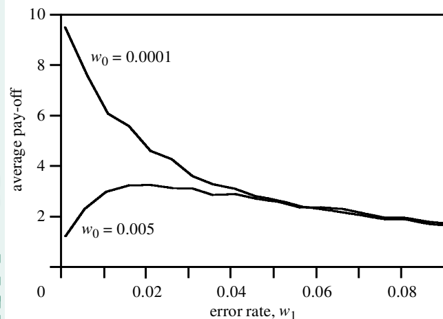
Figure 1. The maximum size of a communication system that can be stably maintained by a population depends on the error rate during language acquisition. Each individual is characterized by a binary association matrix, A , linking arbitrary signals to objects (or concepts). There are n = 10 objects and m = 10 signals. A is a binary 10 \times 10 matrix. The population size is N = 100 . In every generation, each individual talks to every other individual and the pay-offs are summed up. For the next generation, individuals produce offspring who learn their language. The error rate, w_0 , is the probability that a child will have an entry of unity in the A matrix where the parent had a zero entry. Similarly, w_1 is the probability for the child to lose an entry of unity. The figure shows the average pay-off of the population averaged over 5000 generations. The average pay-off is indicative of the number of signals that can be maintained by the population. If all individuals speak a 'perfect' language with n signals referring uniquely to n objects, the average pay-off of the population is n . For w_0 = 0.001 , the average pay-off is a declining function of w_1 . For w_0 = 0.005 , the average pay-off is a one-humped function; for very low w_1 , individuals accumulate too many associations in their A matrix. For a population to maintain a signalling system of size n \times n , both error rates have to be below some critical threshold values.
